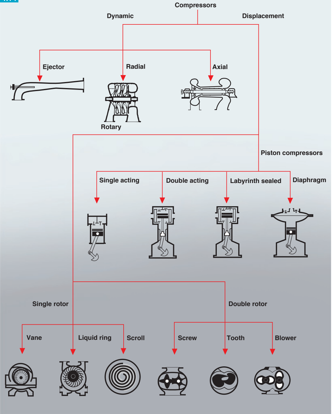
Most common compressor types, divided according to their working principles.
