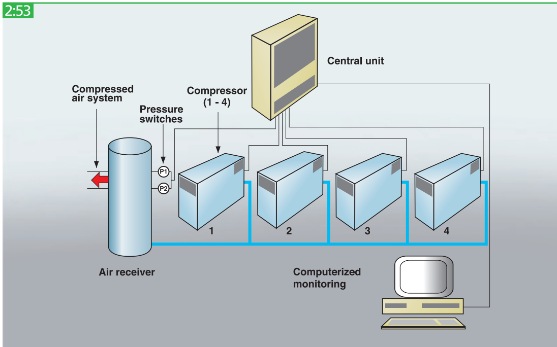
Centrally controlled compressor installation.
